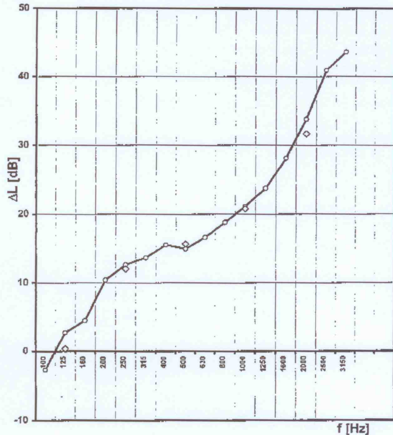
WEIGHTED IMPACT SOUND IMPROVEMENT INDEX
